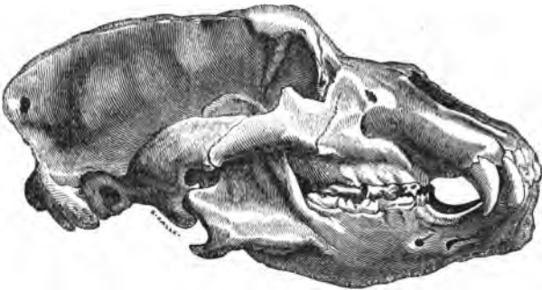
URSUS SPELEUS. Cave Bear. ( Pleistocene. )
